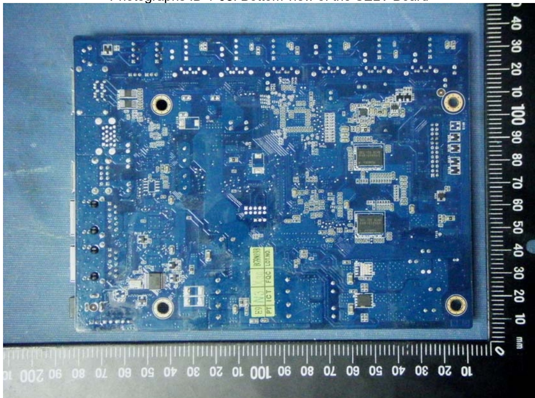
Photographs ID 1-08: Bottom view of the SELV Board
