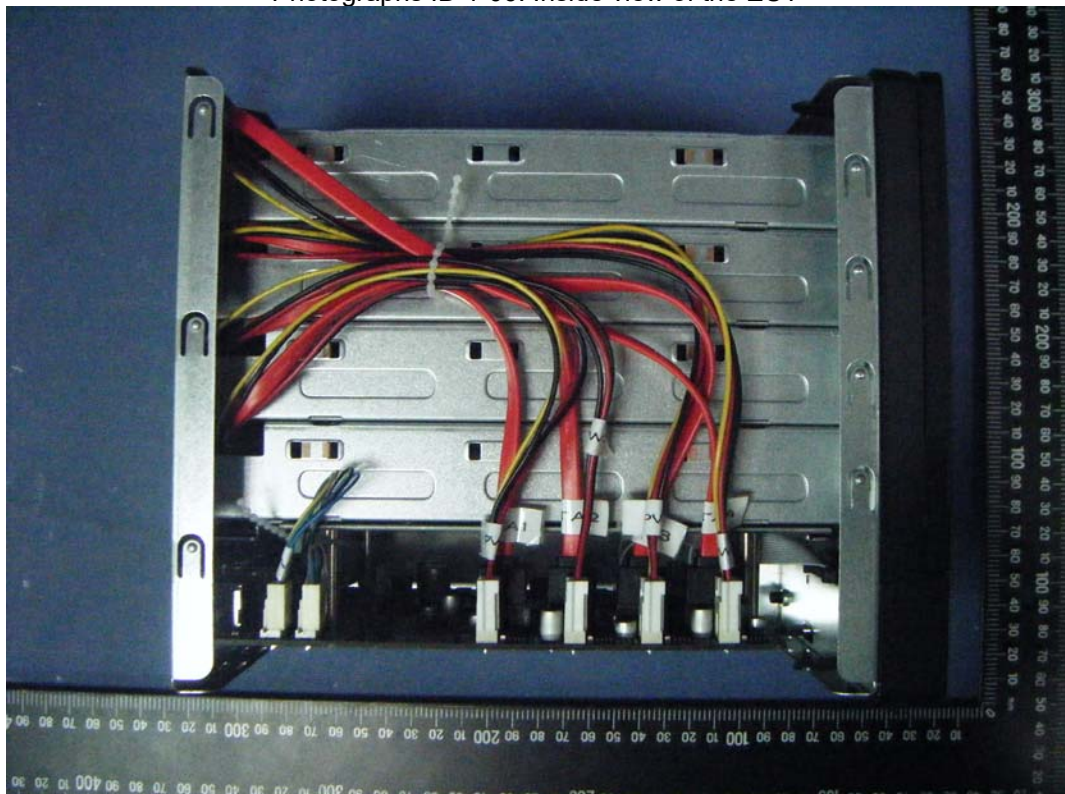
Photographs ID 1-06: Inside view of the EUT
