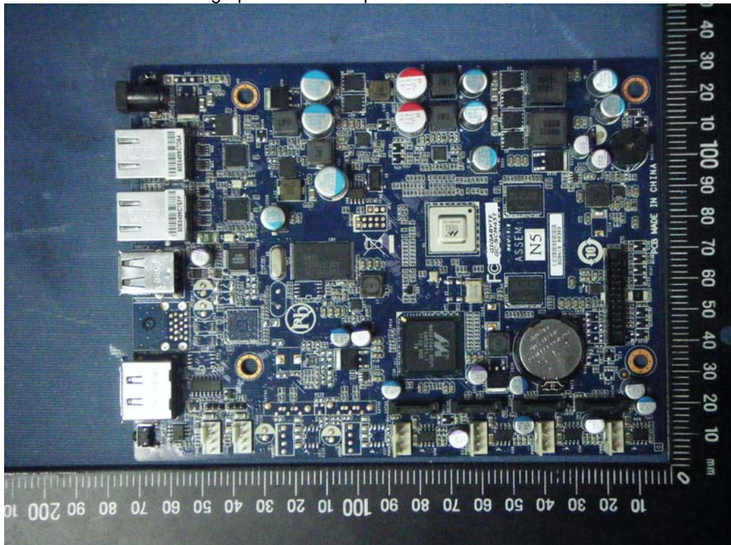
Photographs ID 1-07: Top view of the SELV Board
