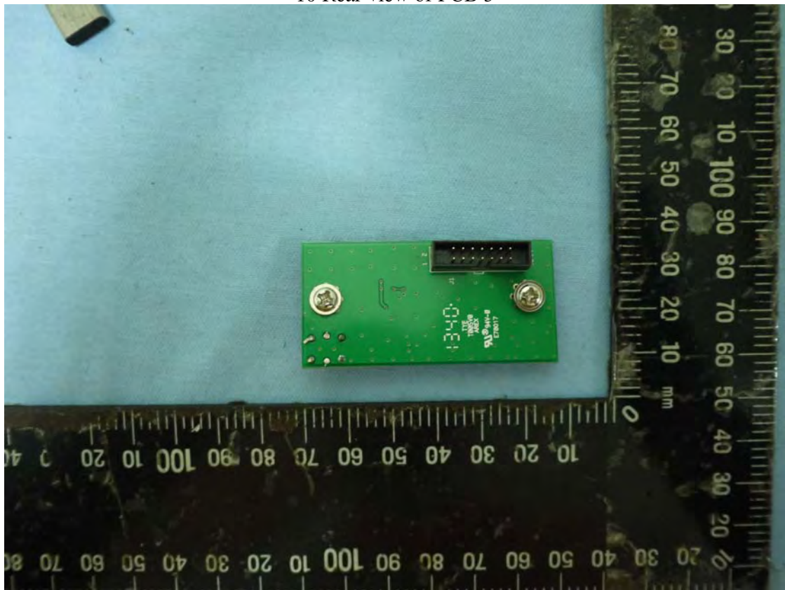
10 Rear view of PCB 3
