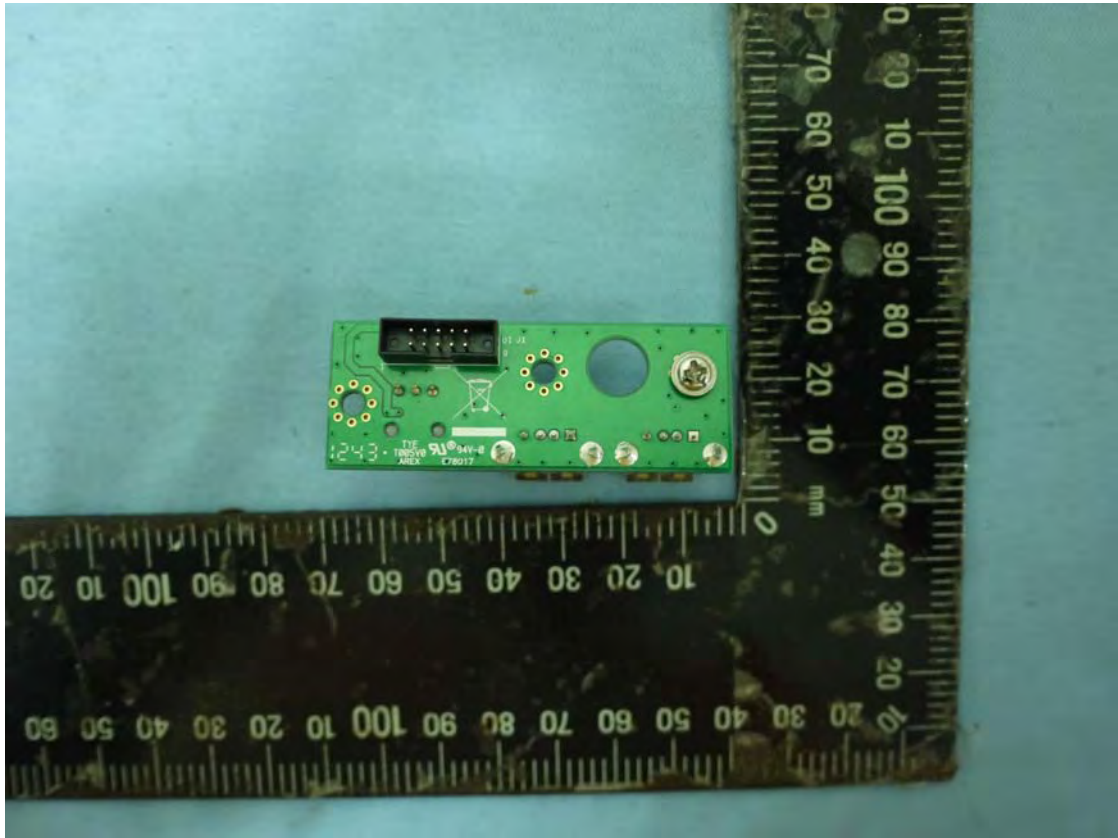
08 Rear view of PCB 2
