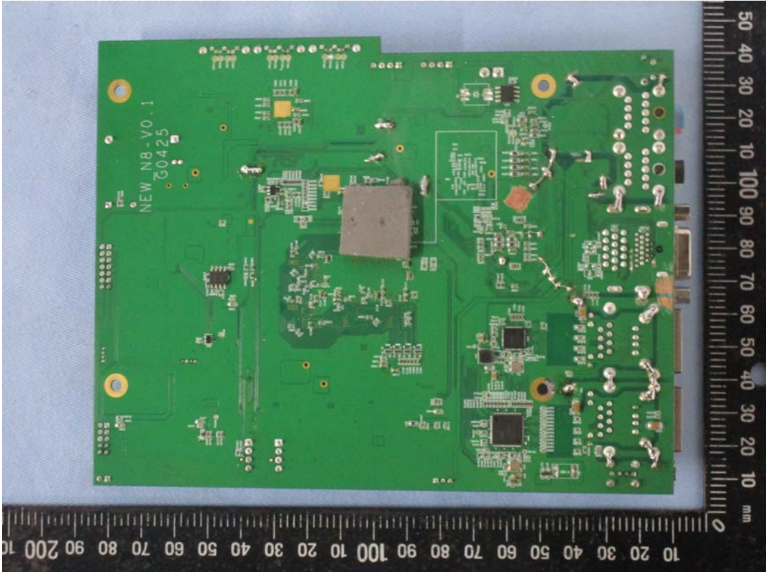
07 Rear View of PCB1
