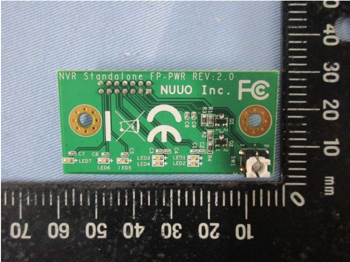
08 Front View of PCB2
