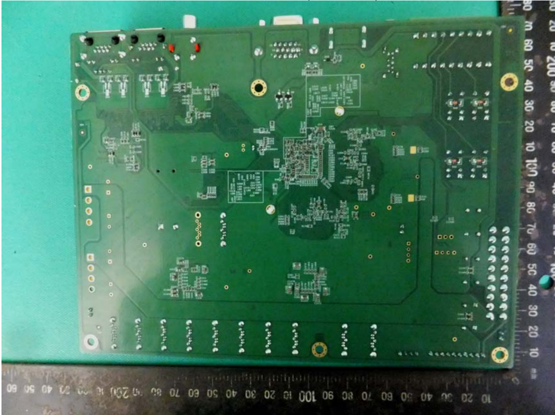
07 Rear view of PCB(Mainboard)
