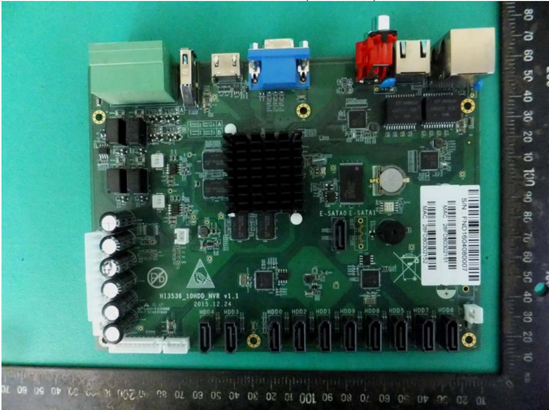
06 Front view of PCB(Mainboard)
