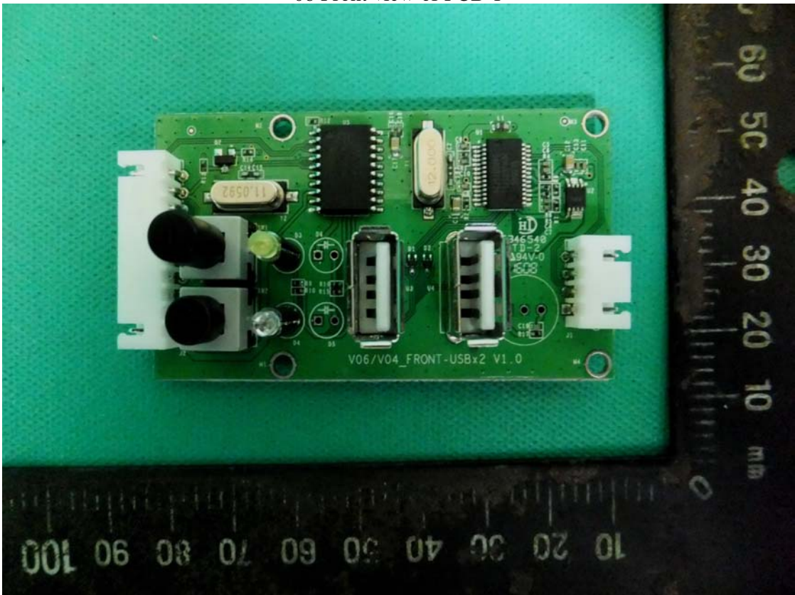
08 Front view of PCB-1
