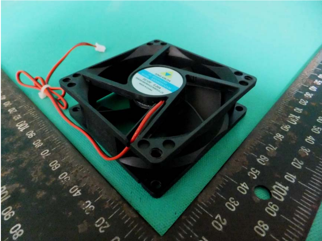
13 View of FAN
